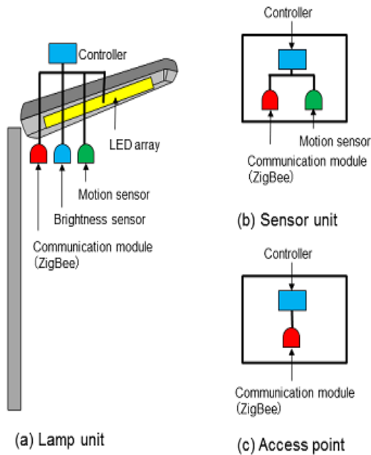
Figure 5: Components for the Smart Street Light [7]
