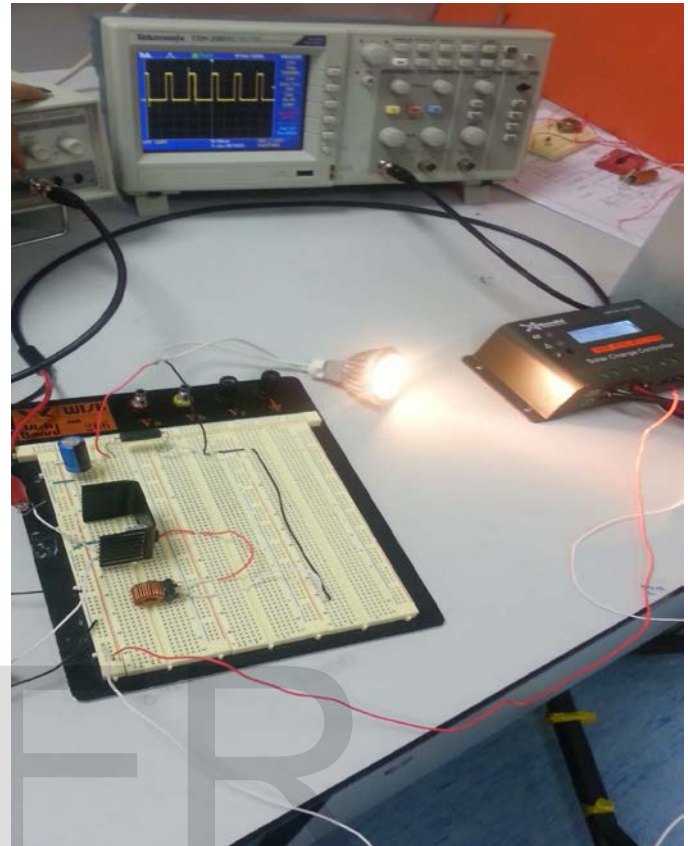
Figure 13: Dimming the 7Watt LED by Varying the Duty Cycle
